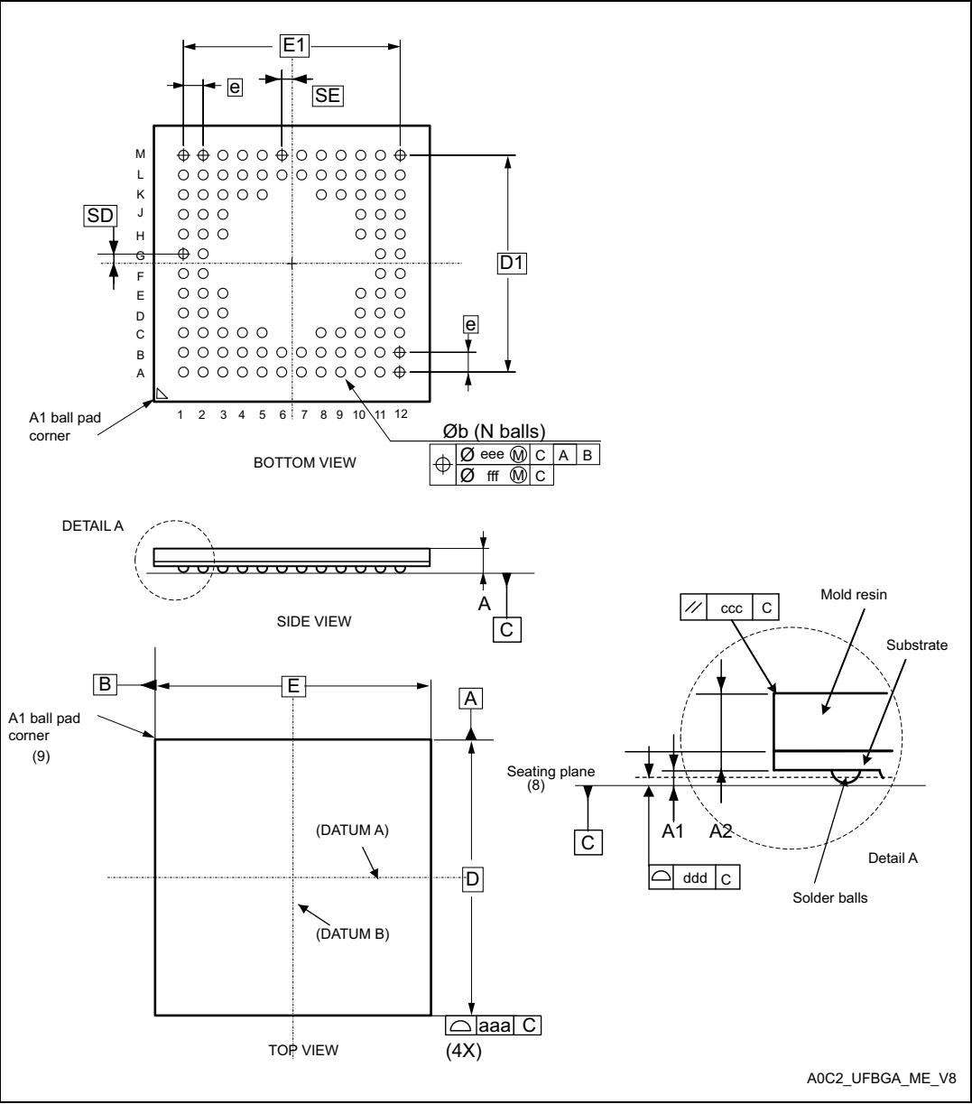
Figure 54. UFBGA100 - Outline (13)
